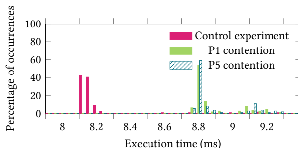
Figure 8: P1 contention experiment on f64.floor for 1 000 000 instructions.
